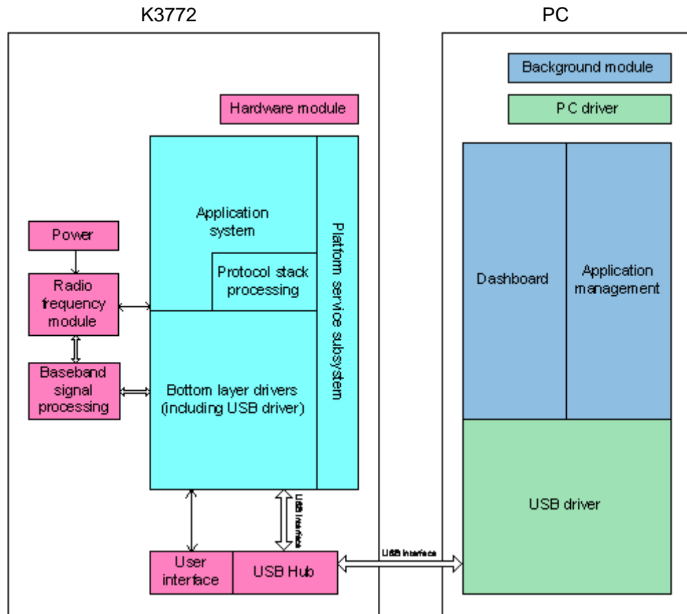
Figure 4-1 System architecture
